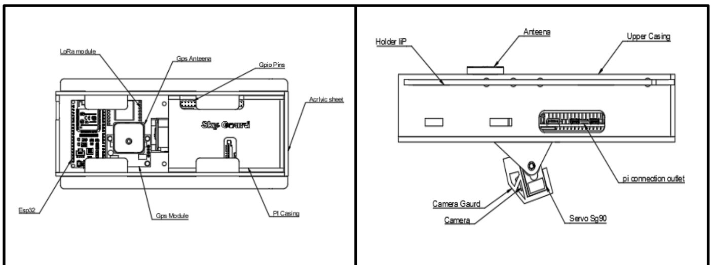
Fig 2.2 Attachment Design
