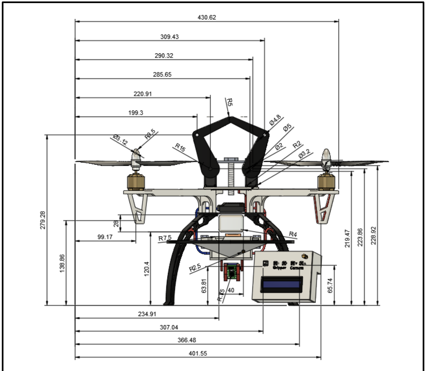
Fig 3.1: Dimensional Render
